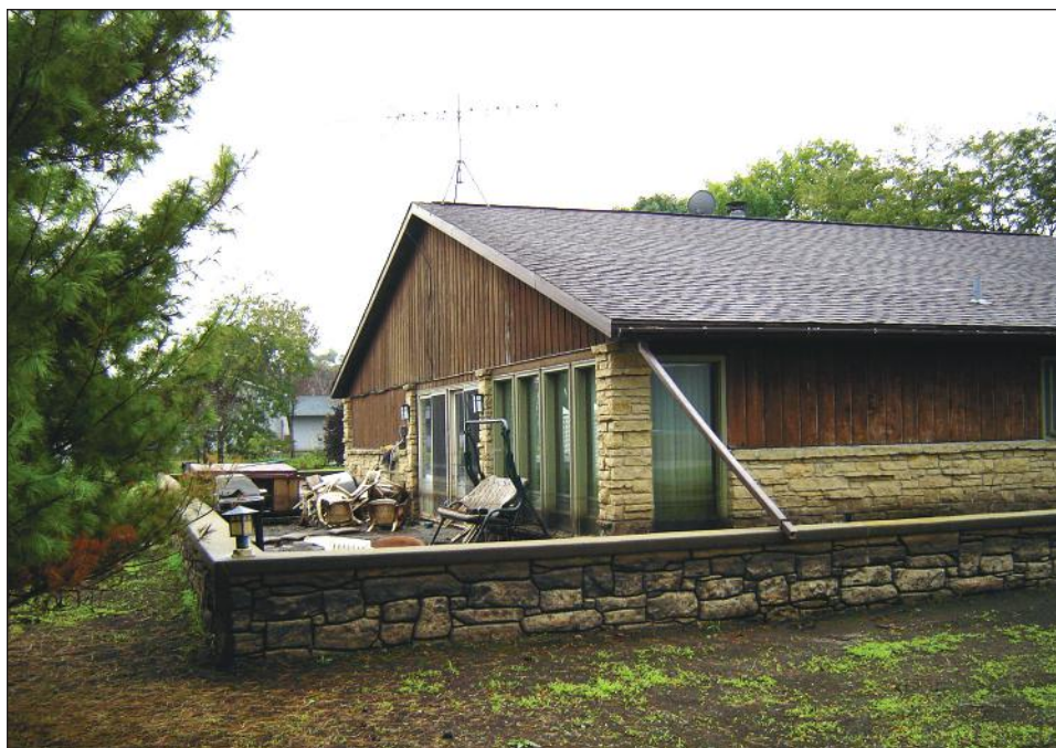
Figure 8-3. Structure protected by a floodwall with decorative stone finish.
